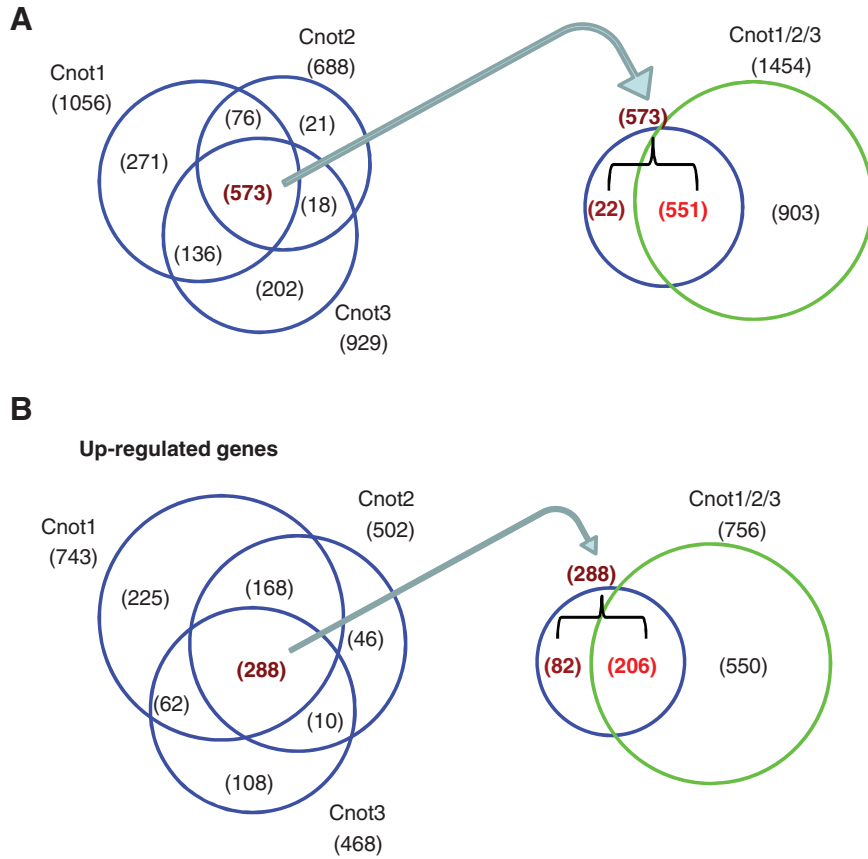
SUPPLEMENTARY FIG. S7. Venn diagrams illustrating the relationships of the effects of overexpression of core components of the Ccr4-Not complex on gene expression profiles of partial iPSCs. (A) Venn diagrams showing genes that were downregulated more than twofold by forced expression of Cnot1, Cnot2 or Cnot3 ( left panel ). Right panel shows the relationship between the 573 genes closed up in the left panel and those with expression levels that were decreased by simultaneous expression of Cnot1, Cnot2, and Cnot3 in partial iPSCs (2B1). (B) Genes upregulated by Cnot1, Cnot2, and Cnot3. Left and right panels show Venn diagrams subjected to the same procedure performed in A with respect to upregulated genes.
