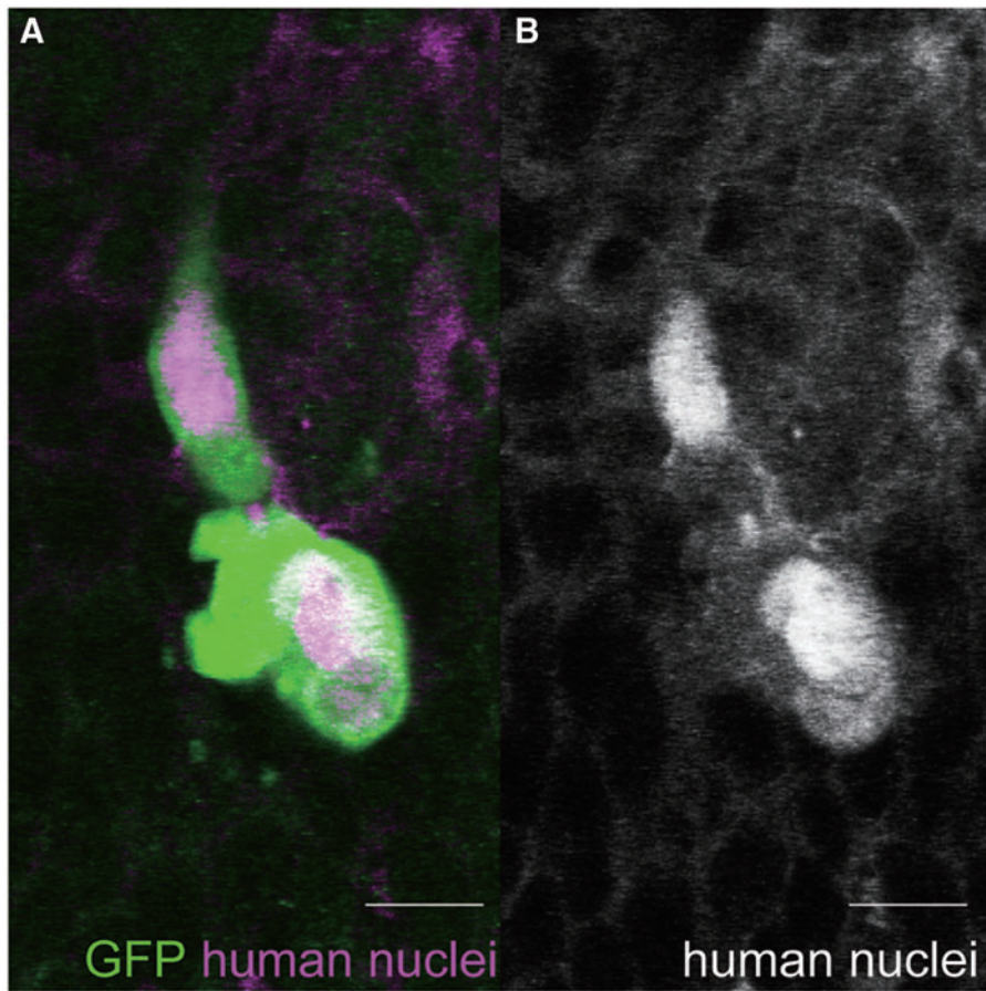
SUPPLEMENTARY FIG. S6. Transplanted human-ESC-derived cells are specifically marked with the anti-all-human nuclei antibody. Grafted human-ESC-derived cells ( A ; green ) 1 day after grafting (E15.5) are labeled with the anti-all-human nuclei antibody ( A ; magenta and B ). GFP-expressing cells are exclusively stained with the anti-human nuclei antibody. Scale bars = 10 \mu m.
