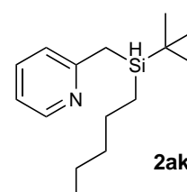
2-(( tert -Butyl(hexyl)silyl)methyl)pyridine
