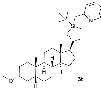
2-(((1 R ,3 R )-1- tert -Butyl-3-((3 R ,5 R ,8 R ,9 S ,10 S ,13 S ,14 S ,17 R )-3-methoxy-10,13-dimethylhexadecahydro-1 H -cyclopenta[ a ]phenanthren-17-yl)silolan-1-yl)methyl)pyridine
