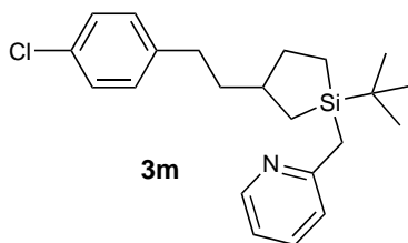
2-((1- tert -Butyl-3-(4-chlorophenethyl)silolan-1-yl)methyl)pyridine
