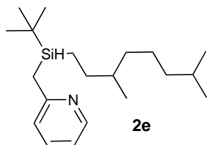
2-(( tert -Butyl(3,7-dimethyloctyl)silyl)methyl)pyridine
