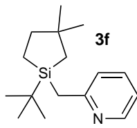
2-((1- tert -Butyl-3,3-dimethylsilolan-1-yl)methyl)pyridine
