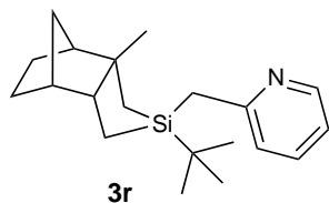
2-[(2- tert -Butyl-3a-methyloctahydro-1 H -4,7-methano-2-benzosilol-2-yl)methyl]pyridine
