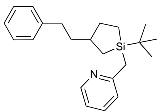
2-((1- tert -Butyl-3-phenethylsilolan-1-yl)methyl)pyridine
