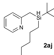
2-(( tert -Butyl(pentyl)silyl)methyl)pyridine
