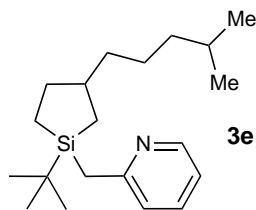
2-((1- tert -Butyl-3-(4-methylpentyl)silolan-1-yl)methyl)pyridine
