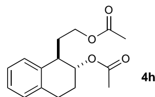
2-(((1 R ( S ),2 R ( S ))-2-Acetoxy-1,2,3,4-tetrahydronaphthalen-1-yl) ethyl acetate
