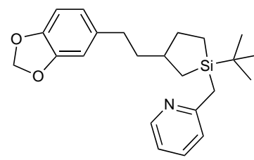
2-((3-(2-(Benzo[ d ][1,3]dioxol-5-yl)ethyl)-1- tert -butylsilolan-1-yl)methyl)pyridine
