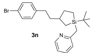
2-((1- tert -Butyl-3-(4-bromophenethyl)silolan-1-yl)methyl)pyridine
