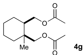
(1-Methylcyclohexane-1,2-diyl) dimethanediyl diacetate
