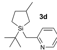
2-((1- tert -Butyl-3-methylsilolan-1-yl)methyl)pyridine
