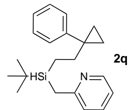
2-(( tert -Butyl(2-(1-phenylcyclopropyl)ethyl)silyl)methyl)pyridine
