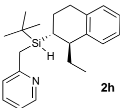
2-(( tert -Butyl(1-ethyl-1,2,3,4-tetrahydronaphthalen-2-yl)silyl)methyl)pyridine
