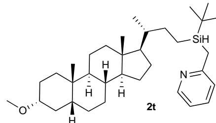
2-(( tert -Butyl(( R )-3-((3 R ,5 R ,8 R ,9 S ,10 S ,13 R ,14 S ,17 R )-3-methoxy-10,13-dimethylhexadecahydro-1 H -cyclopenta[ a ]phenanthren-17-yl)butyl)silyl)methyl)pyridine
