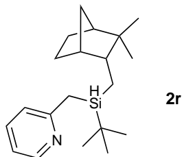
2-(( tert -Butyl((3,3-dimethylbicyclo[2.2.1]heptan-2-yl)methyl)silyl)methyl)pyridine
