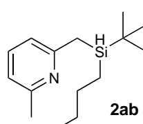
2-(( tert -Butyl(butyl)silyl)methyl)-6-methylpyridine
