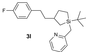
2-((1- tert -Butyl-3-(4-fluorophenethyl)silolan-1-yl)methyl)pyridine
