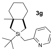
2-((2- tert -Butyl-3a-methylocta-hydro-1 H -benzo[ c ]silol-2-yl)methyl)pyridine
