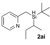
2-(( sec -Butyl( tert -butyl)silyl)methyl)pyridine
