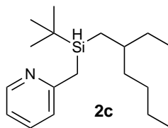
2-(( tert -Butyl(2-ethylhexyl)silyl)methyl)pyridine
