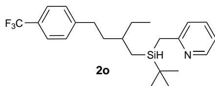
2-(( tert -Butyl(2-ethyl-4-(4-(trifluoromethyl)phenyl)butyl)silyl)methyl)pyridine
