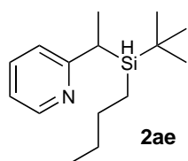
2-(1-( tert -Butyl(butyl)silyl)ethyl)pyridine
