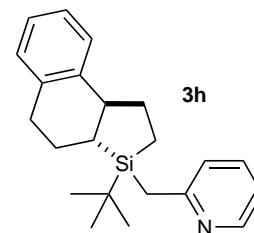
2-(((3 S ,3 aR ,9 bR )-3-( tert -butyl)-2,3,3 a ,4,5,9 b -hexahydro-1 H -naphtho[2,1- b ]silol-3-yl)methyl)pyridine
