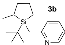
2-((1- tert -Butyl-2-methylsilolan-1-yl)methyl)pyridine
