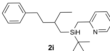
2-(( tert -Butyl(2-ethyl-4-phenylbutyl)silyl)methyl)pyridine
