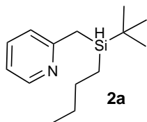
2-(( tert -Butyl(butyl)silyl)methyl)pyridine
