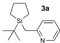
2-((1- tert -Butylsilolan-1-yl)methyl)pyridine
