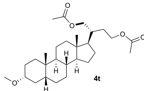
( R )-2-((3 R ,5 R ,8 R ,9 S ,10 S ,13 S ,14 S ,17 R )-3-Methoxy-10,13-dimethylhexadecahydro-1 H -cyclopenta[ a ]phenanthren-17-yl) butane-1,4-diyl diacetate
