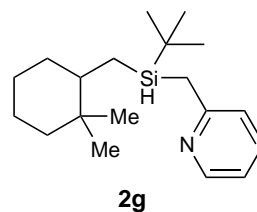
2-(( tert -Butyl((2,2-dimethylcyclohexyl)methyl)silyl)methyl)pyridine
