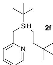
2-(( tert -Butyl(3,3-dimethylbutyl)silyl)methyl)pyridine
