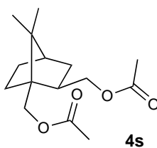
[(1 R ,2 R ,4 R )-7,7-dimethylbicyclo[2.2.1]heptane-1,2-diyl] di(methylene) diacetate
