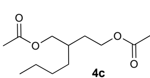
2-Butylbutane-1,4-diyl diacetate
