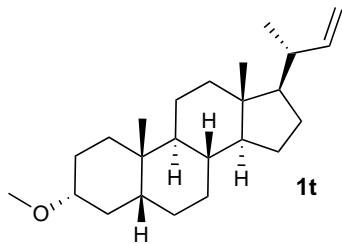
3 \alpha -Methyl-24-nor-5 \beta -chol-22-ene
