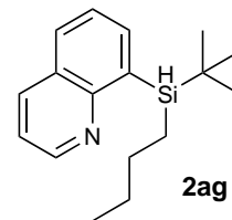
8-( tert -Butyl(butyl)silyl)quinolone
