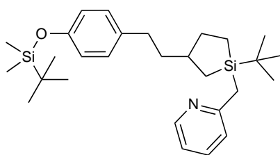
2-((1- tert -Butyl-3-(4-( tert -butyl)dimethylsilyloxy)phenethyl)silolan-1-yl)methyl)pyridine
