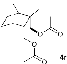
[(1 S ( R ),2 S ( R ),3 R ( S ),4 R ( S ))-2-methylbicyclo[2.2.1]heptane-2,3-diyl] di(methylene) diacetate
