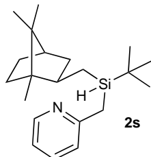
2-(( tert -Butyl((1,7,7-trimethylbicyclo[2.2.1]heptan-2-yl)methyl)silyl)methyl)pyridine
