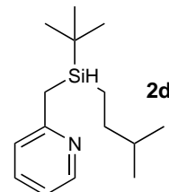
2-(( tert -Butyl(isopentyl)silyl)methyl)pyridine
