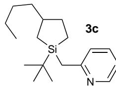
2-((1- tert -Butyl-3-butylsilolan-1-yl)methyl)pyridine
