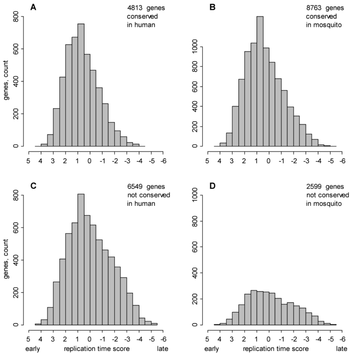
Supplementary fig. S1. Replication timing for genes on chromosomes 2 and 3 in C18 cells. (A) Genes with homologs in the human genome. (B) Genes with homologs in the mosquito genome. (C) Genes without human homologs. (D) Genes without mosquito homologs.
