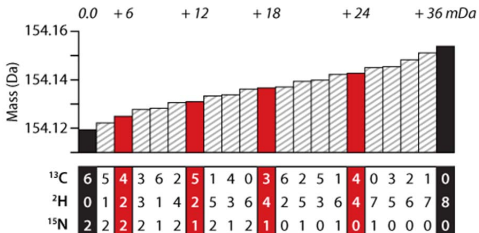
Supplemental Figure 1. Theoretical mass calculations of the 21 isotopologues for an M+8 lysine amino acid. Shown in solid black are the isotopologues that are commercially available. Shown in red are the novel isotopologues synthesized for the experiments presented here.
