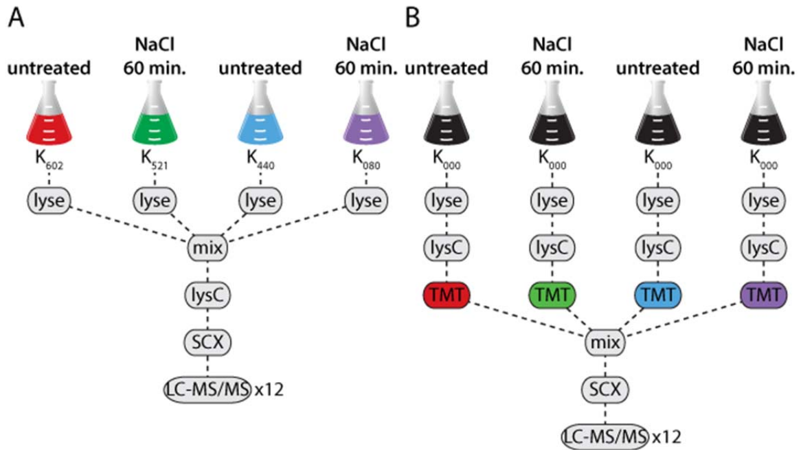
Supplemental Figure 2. Four-plex (a) NeuCode SILAC and (b) TMT workflows for yeast salt stress experiments.
