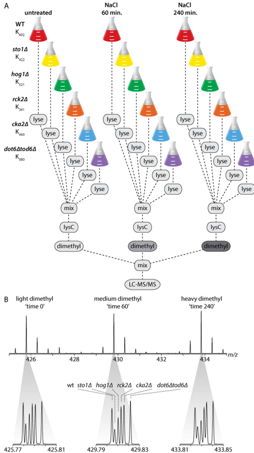
Supplemental Figure 3. 18-plex NeuCode SILAC for expanded yeast salt stress experiments. (a) Experimental workflow. (b) Dimethyl labeling creates a maximum of three isotopic clusters (i.e., time points). NeuCode SILAC labeling creates a maximum of six isotopologue peaks (i.e., strains) within each isotopic cluster.
