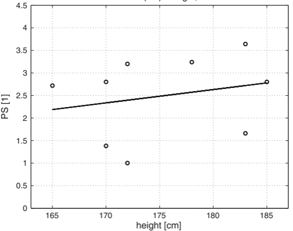
Platform Score (PS) - height, R=0.228
