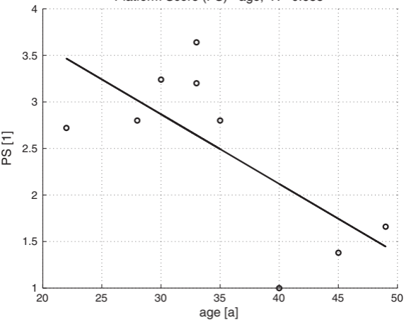
Platform Score (PS) - age, R=-0.688
