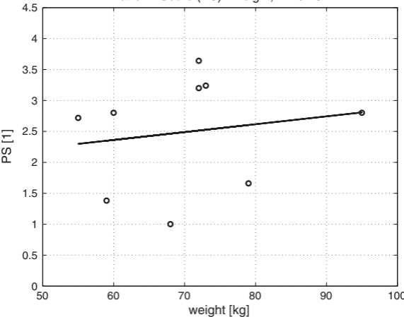
Platform Score (PS) - weight, R=0.167
