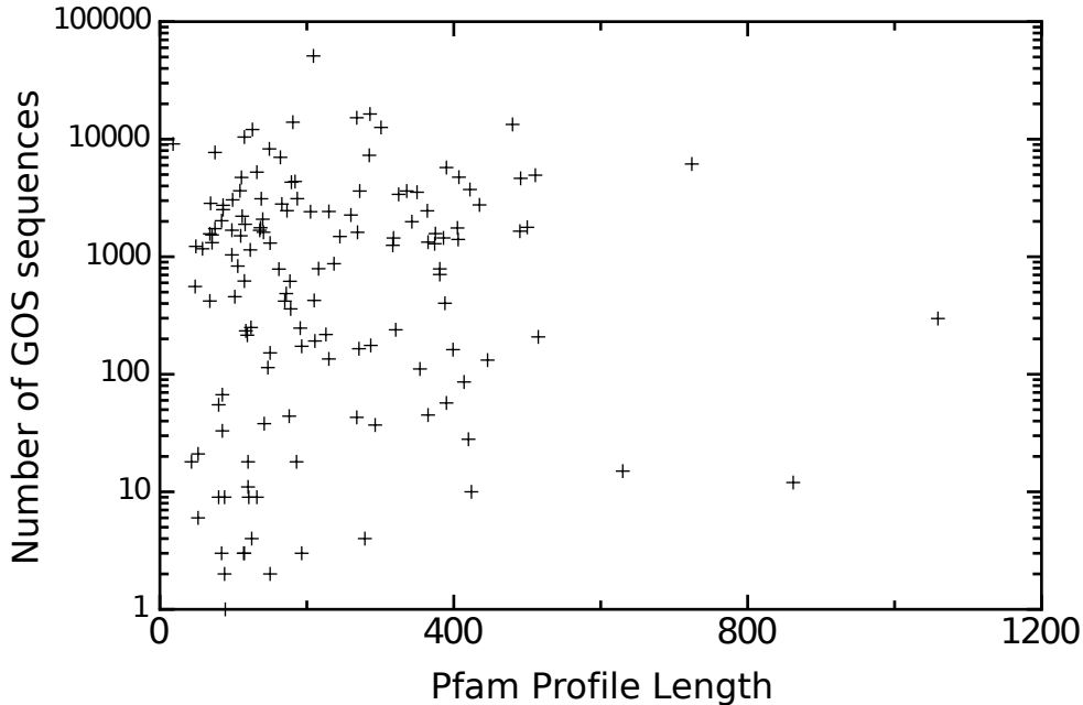
Profile length versus found sequences
