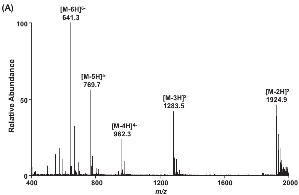
Figure S1. Negative-ion ESI-MS of the standard ODN harboring a 5-gHmdC (A) and the product-ion spectrum of the [M-3H]^{3-} ion (B).
