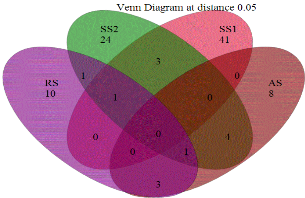
(a) cbbM
