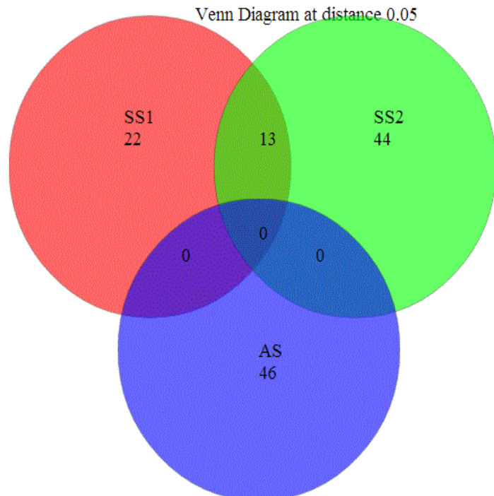
(c) soxB
