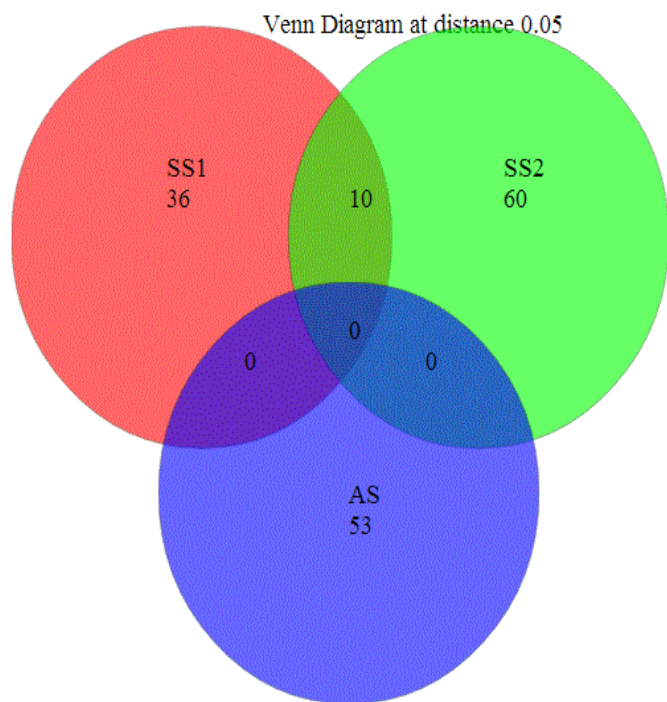
(b) apsA
