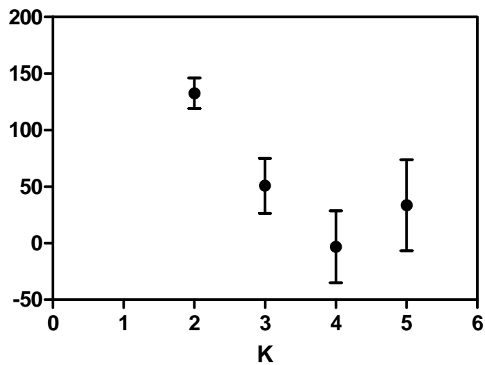
B. \ln' \Pr(X|K)
