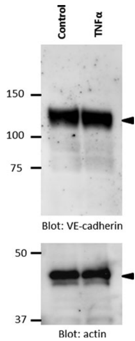
SUPPLEMENTARY FIG. S2. Western analysis for VE-cadherin in TNF- \alpha -treated cells. The total amount of VE-cadherin was not altered by TNF- \alpha stimulation. VE-cadherin was detected as one band of 130 kDa ( arrow ) in the upper blot . The lower blot showed one band of actin at 45 kDa ( arrow ) as control. The blots were representative of three separate experiments.
