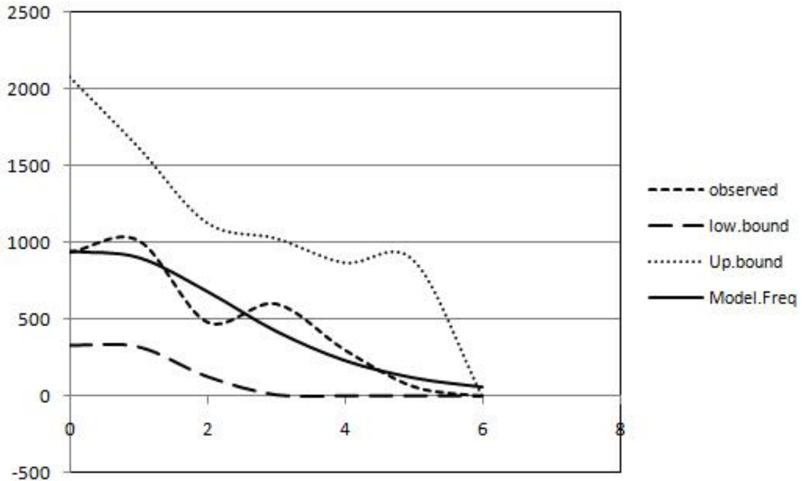
Figure S4 Mismatch distribution based on the pairwise differences between individuals. The observed distribution of the sequence mismatches was multimodal, which corresponds to a stable population, the modeled curve showed a smooth distribution characteristic for expanding populations.
