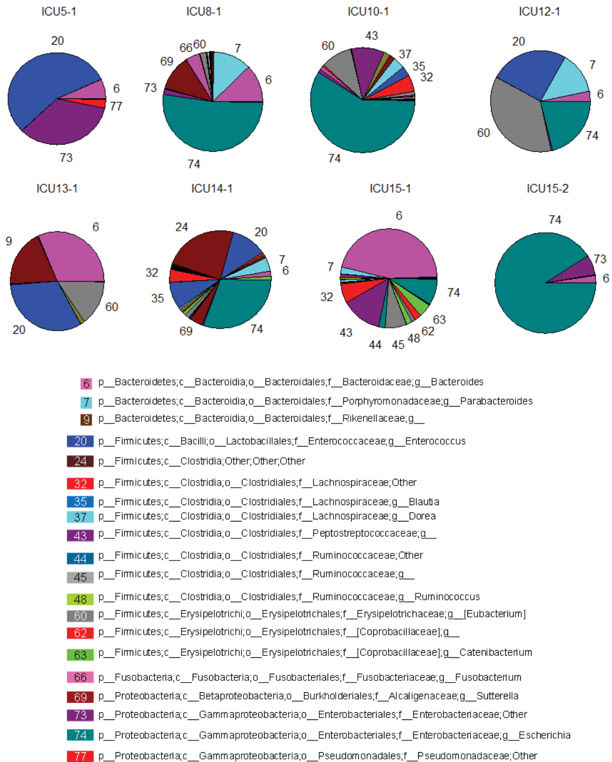
Supplemental Fig.S3. The taxonomic composition of gut microbiome in stool samples with the decreased bacterial diversity. Escherichia (#74) and Enterococcus (#20) were major pathogens in this group.
