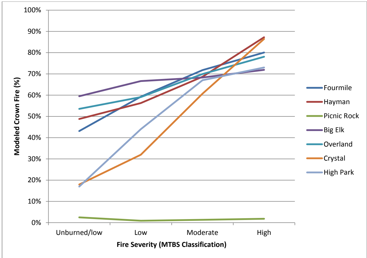
Figure S2. MTBS fire severity class (observed) and percentage of crown fire (modeled).
