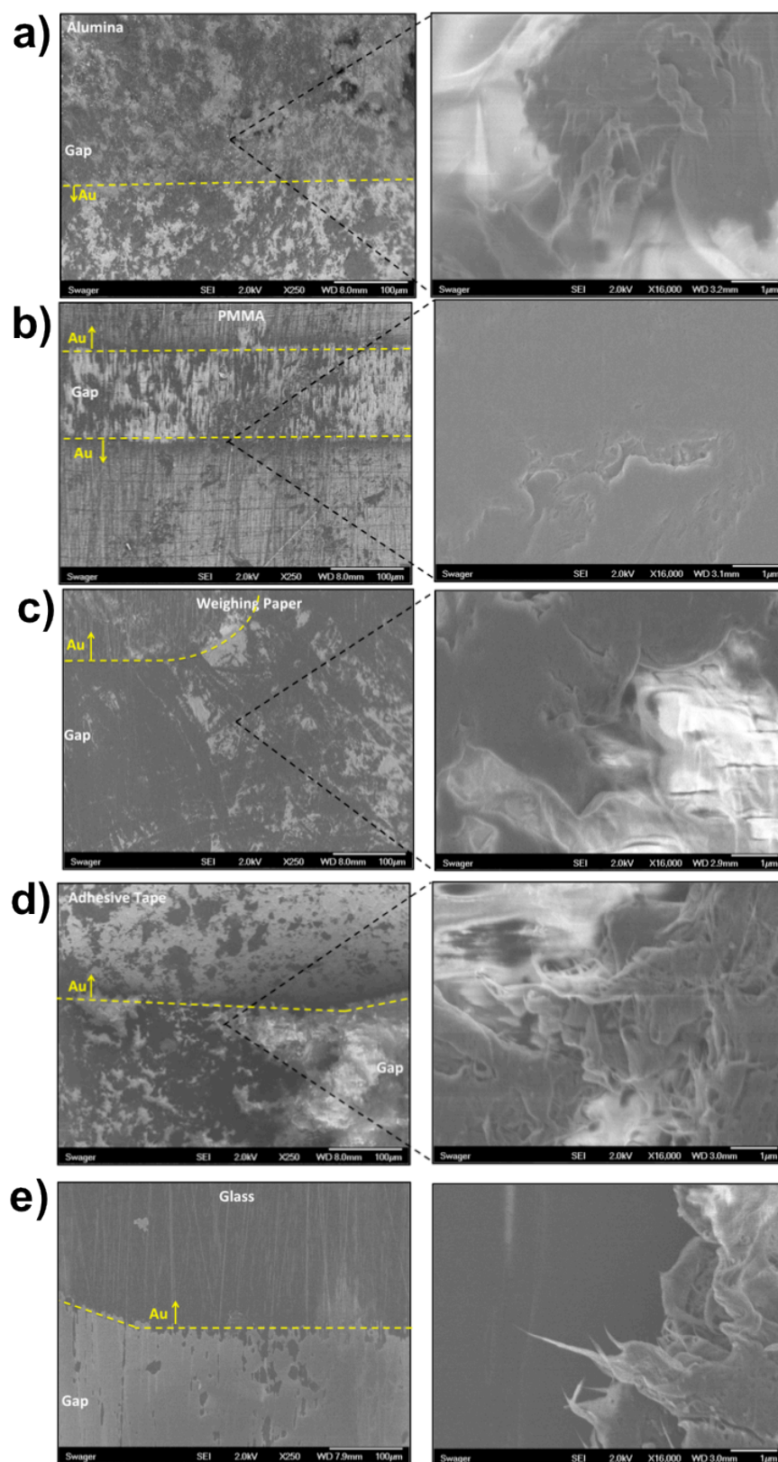
Figure S3. Characterization of abraded films of sensing materials using high resolution Scanning Electron Microscopy (SEM). a-e) Images of compressed pristine SWCNTs deposited by abrasion between and on top of gold electrodes onto alumina, PMMA, weighing paper, adhesive tape, and glass, respectively.
