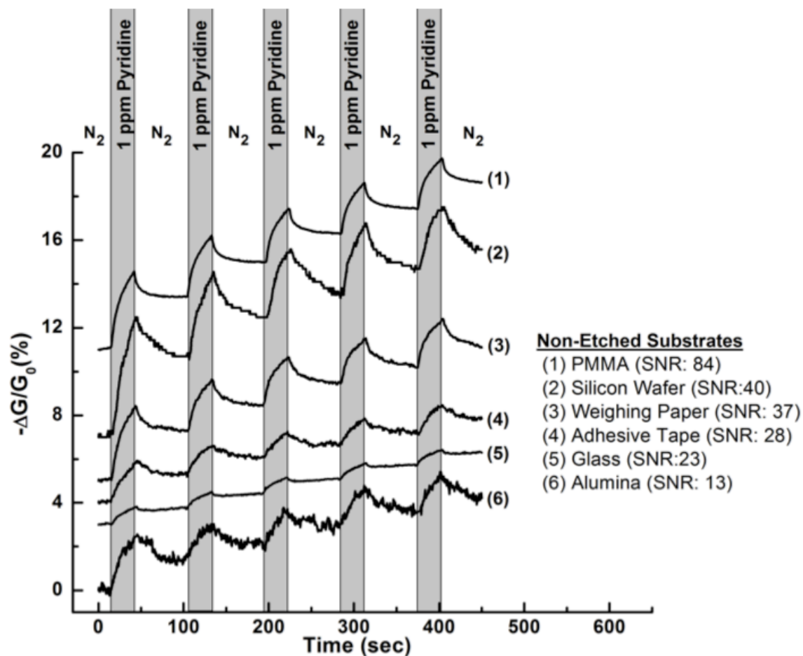
Figure S8. Investigation of the SWCNT-based chemiresistor's sensitivity on various unmodified substrates. Normalized change of conductance over time from devices simultaneously exposed five consecutive times to 1 ppm pyridine for 30 s with a recovery time of 60s. Devices were fabricated by depositing SWCNT:TEC (2:1 mass ratio) on top of and between gold electrodes by abrasion onto various substrates.
