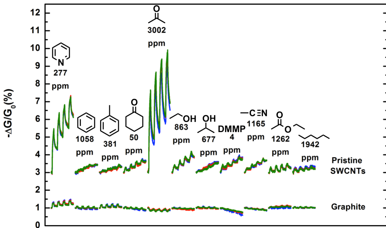
Figure S12. Comparison of sensing responses from graphite and pristine SWCNTs deposited on the surface of weighing paper between gold electrodes. Resistance range of the sensors was between 1-2 k \Omega . Normalized change of conductance over time for three devices simultaneously exposed four consecutive times to various analytes for 30 s with a recovery time of 60 s.
