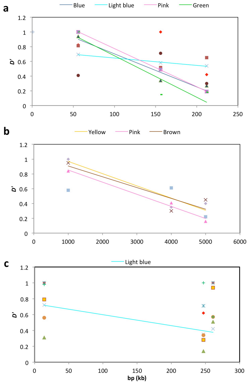
Supplementary Figure S2. Relationship between pair-wise linkage disequilibrium and the physical distance between markers on three supercontigs in the genetic clusters inferred by Bayesian posterior probability clustering. Trend lines were shown only to those R^2 > 0.5 . a). Supercontig 3 (Chromosome 4); b) Supercontig 9 (Chromosome 6); and c) Supercontig 19 (Chromosome 5).
