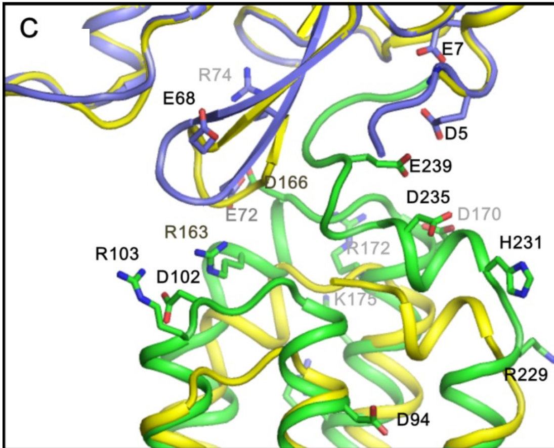
Figure S3. pH dependence of the structure of cR3 in the cytoplasmic and extracellular surface regions. The protein structure observed at pH 5 (green and blue) is compared with that observed at pH 6 (yellow). The inter-membrane space in the P321 crystal expanded significantly in the post-crystallization soaking solution at pH 6.
