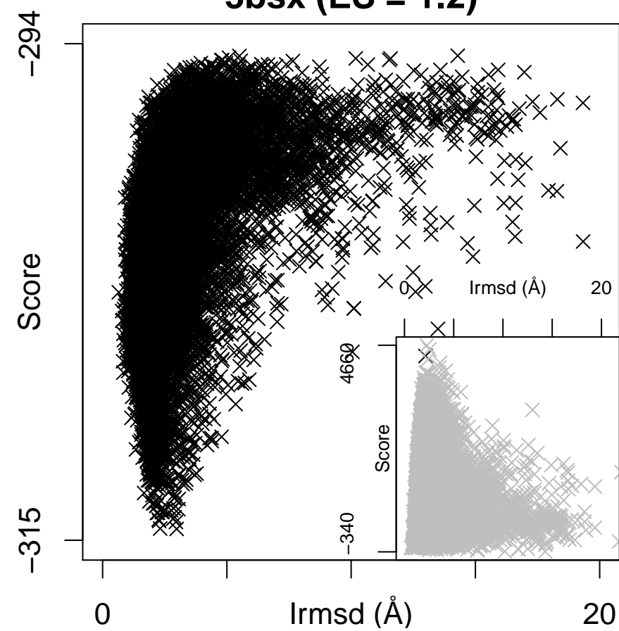
3bsx (ES = 1.2)
