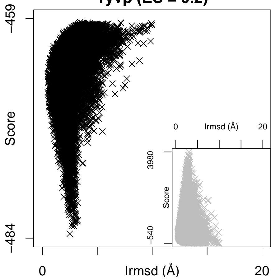
1yvp (ES = 0.2)
