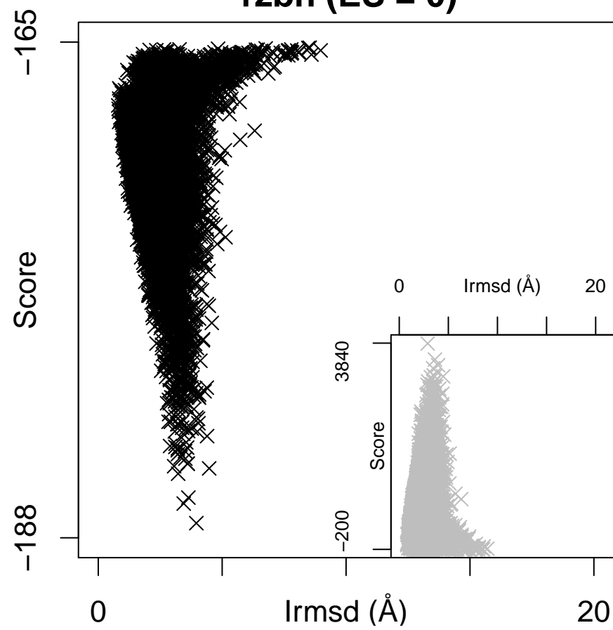
1zbh (ES = 0)
