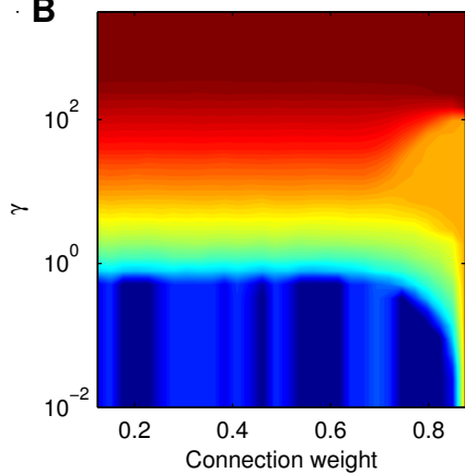
small world
