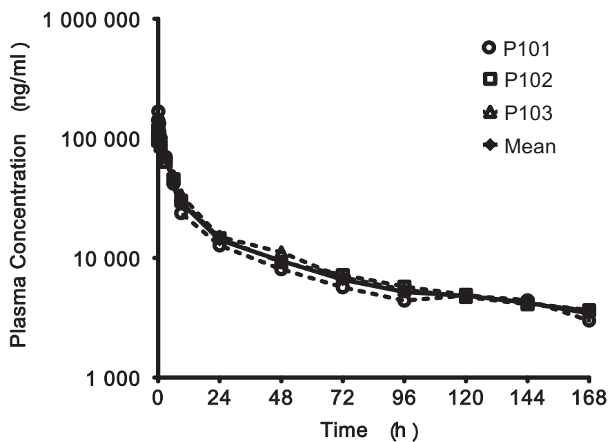
Supplementary Figure S3 Individual and mean plasma concentrations versus time profile of suramin following intravenous bolus administration of suramin at 4.37 mg/kg to male cynomolgus monkeys. Three monkeys were included, and were labeled as P101, P102 and P103 respectively.
