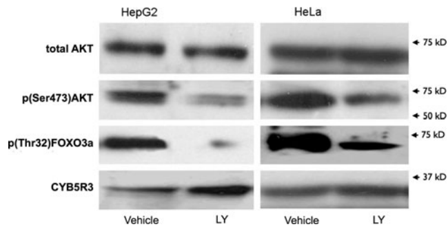
SUPPLEMENTARY FIG. S2. Evaluation of CYB5R3 expression in HepG2 and HeLa cells. HepG2 and HeLa cells were treated with LY294002 (LY) for 12 h and then lysed. Western blotting was performed using antibodies against phospho-AKT, phospho-FOXO3a, and CYB5R3. Membranes were reprobbed for total AKT, which served as a loading control. FOXO3a, forkhead box class O 3a; AKT, v-akt murine thymoma viral oncogene homolog 1.
