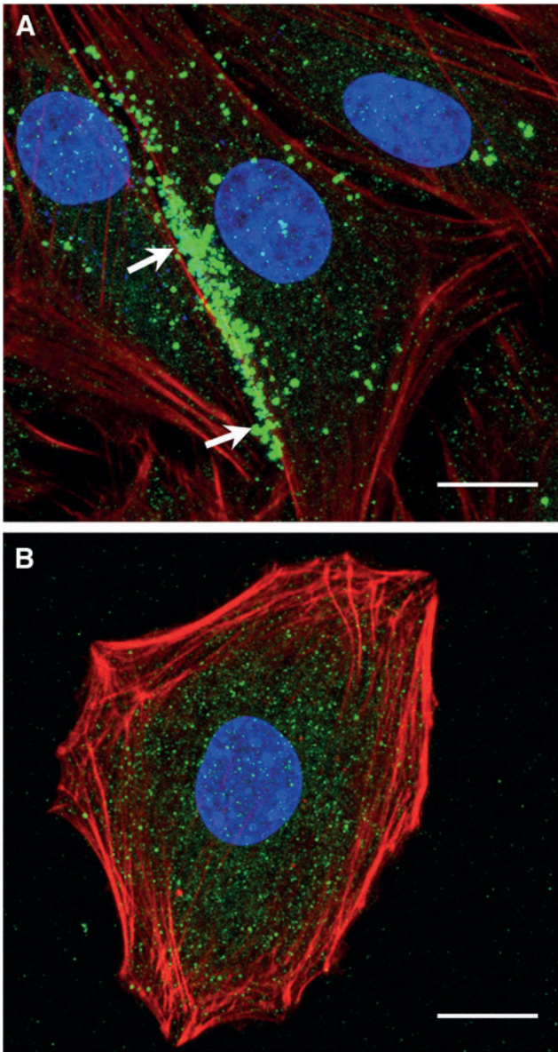
SUPPLEMENTARY FIG. S1. Immunofluorescent confocal microscopy showing endogenous C12orf29 expression in sheep periodontal ligament and MC3T3-E1 cells. (A) Cells isolated from the periodontium of sheep show high expression of C12orf29 in the cytosol. The concentration is particularly strong along a ridge near the cell surface indicated by arrows. This feature is indicative of accumulation in the endoplasmic reticulum and that the protein is being exported out of the cells. (B) A MC3T3-E1 cell showing high C12orf29 expression in a punctate pattern within the cytosol. Scale bars = 20 \mu\text{m} .
