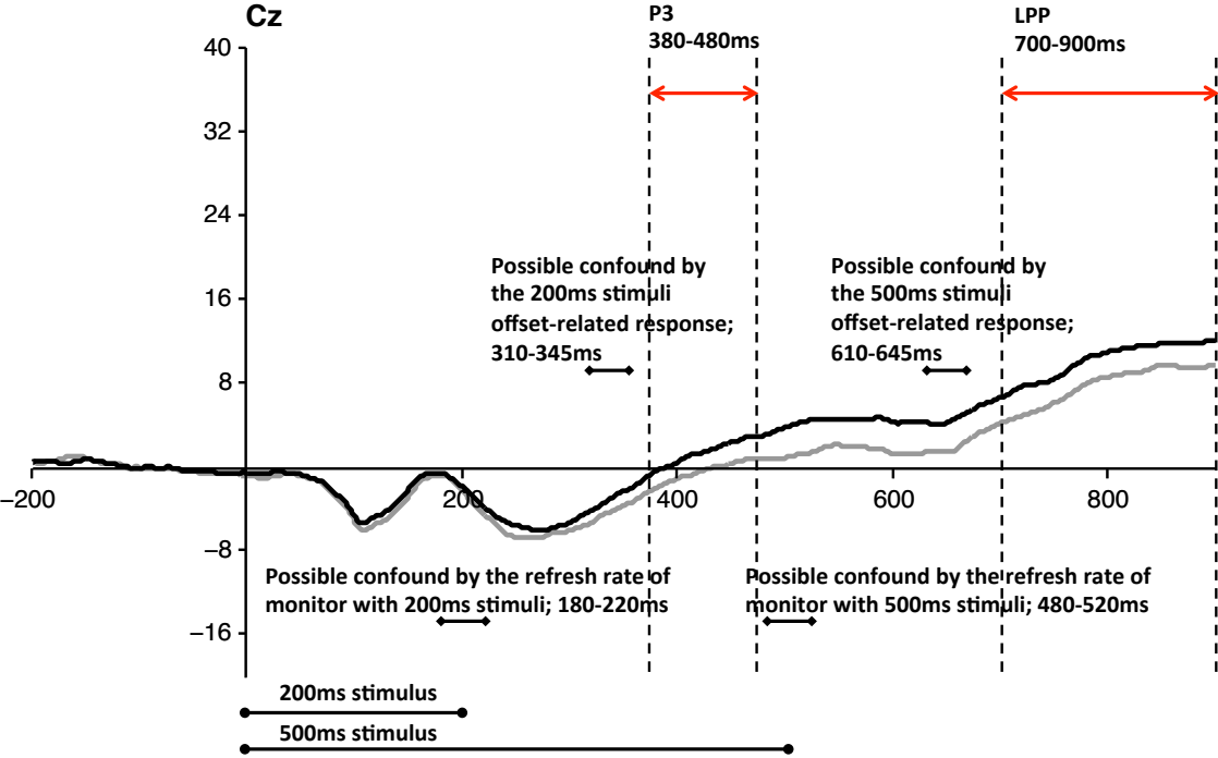
Supplemental Figure 2. Sample waveform for explaining the time epochs we applied in this paper.
