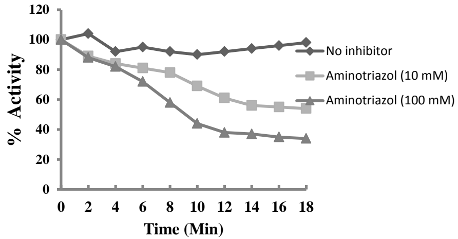
Fig S2: Activity of purified LdAPx against Aminotriazol
