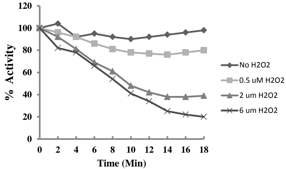
Fig S1: Activity of purified LdAPx against H 2 O 2
