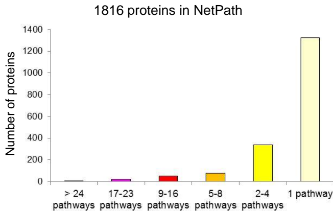
Supplementary Figure S2. Participation of 1816 proteins in 33 Netpath signaling pathways. (A) In the network (upper part), the colour and size of the nodes represents the number of signalling pathways they predicate in (see legend). (B) Graph showing the number of participating proteins in different pathways for all 1816 proteins in NetPath. (C) Graph showing the number of participating proteins (divided by the total number of proteins in each category from panel A) for the 15 proteins involved in RASopathies.
