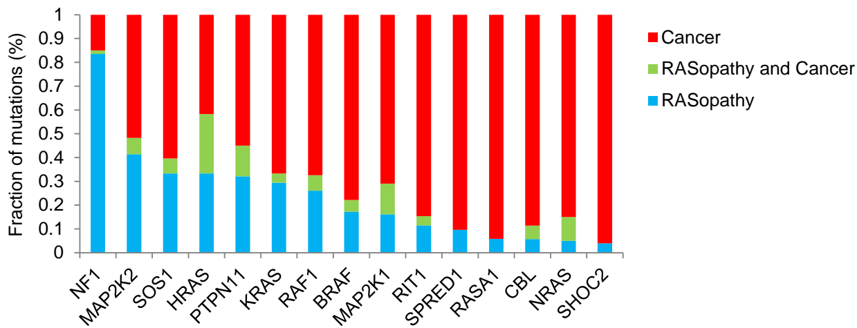
Supplementary Figure S6. Fraction of different RASopathy and cancer mutations in each of the 15 genes.
