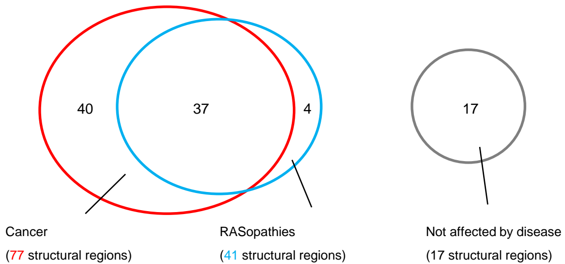
Supplementary Figure S7. Summary of the distribution of somatic and germline mutations in 98 different structural domains and inter-structural regions. Summary of the co-occurrence of germline and RASopathy mutations in different structural regions as shown in Figure 2.
