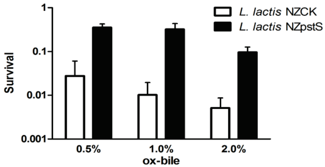
Fig. S4. Enhanced bile survival conferred by bifidobacterial pstS on L. lactis NZ9000. Survival is calculated as the ratio of the number of colonies obtained on GM17 plates after and before different concentrations of ox-bile challenge. Data are mean \pm standard deviation of three independent experiments.
