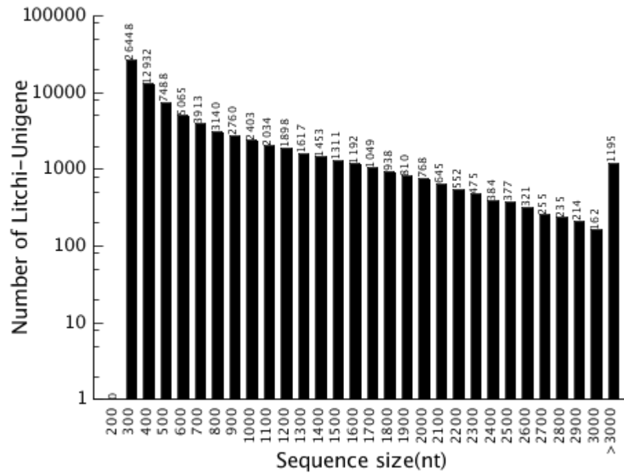
Length distribution of Litchi-Unigene
