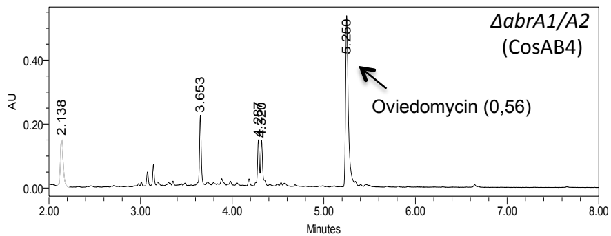
Figure S3: Ovidomycin UPLC profiles production. UPLC profiles of S. coelicolor M145 and S. coelicolor \Delta abrA1/A2 harbouring pKC505 (empty vector) or CosAB4 (containing ovidomycin cluster) Ovidomycin peak is marked with an arrow and the peak height is shown in brackets
