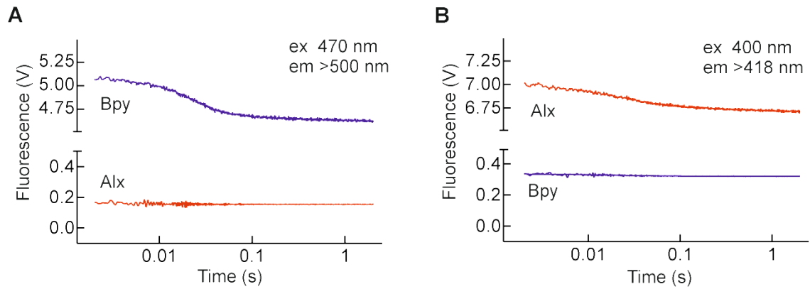
Supplementary Figure S1 Independent monitoring of Bpy (50S TL, blue) and Alx (30S TL, red) fluorescence changes upon addition of EF-G to single-labeled PRE complexes. (A) At emission and excitation wavelengths for Bpy acquisition. (B) At emission and excitation wavelengths for Alx acquisition.
