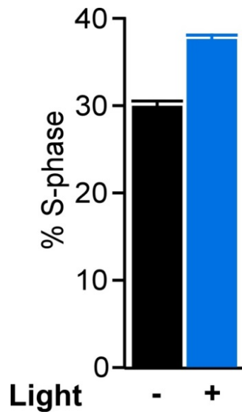
Figure S10. Percentage of M38K Opto-mFGFR1 cells in S-phase in response to blue light. Cells were stimulated with blue light for 1 h. Cell cycle was analysed after 24 h by flow cytometry. Light intensity was \sim 2.5 \mu\text{W}/\text{mm}^2 . Mean values \pm SEM for two independent experiments each performed in triplicates are shown.
