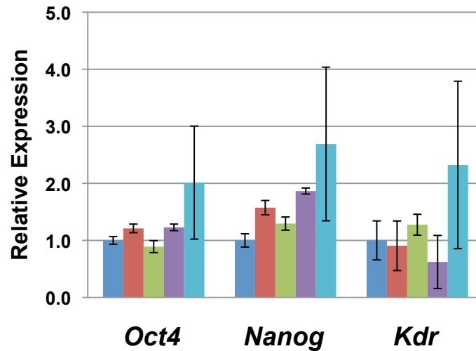
Figure S28. The effect of CPSF30 and CFIm25 depletion on APA and ESC. (A) aUTR RT-qPCR results 3 days after ESCs are transfected with the specified siRNAs are normalized to siCtrl and plotted as mean \pm SEM (n=3). (B) RT-qPCR analyses of ESC ( Oct4 and Nanog ) and differentiation marker ( Kdr ) in the same samples used in (A). Expression values are normalized to siCtrl and plotted as mean \pm SEM (n=3).
