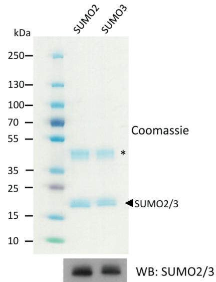
Figure S3. Comparable affinity of the anti-SUMO2/3 antibody to SUMO2 and SUMO3 proteins. Same amount of purified unconjugated SUMO2 and SUMO3 proteins were separated on SDS-PAGE gel and proteins were detected by Coomassie staining (upper) and Western blotting (lower) using the anti-SUMO2/3 antibody. *, unknown protein.
