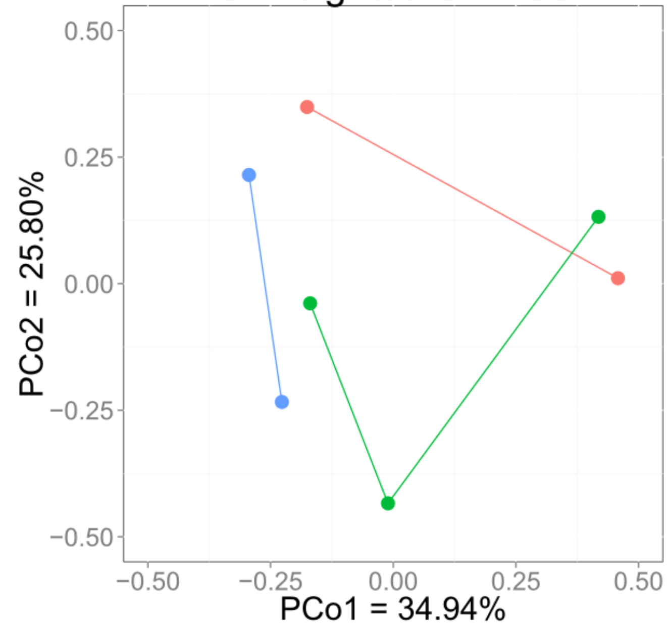
Unweighted UniFrac
