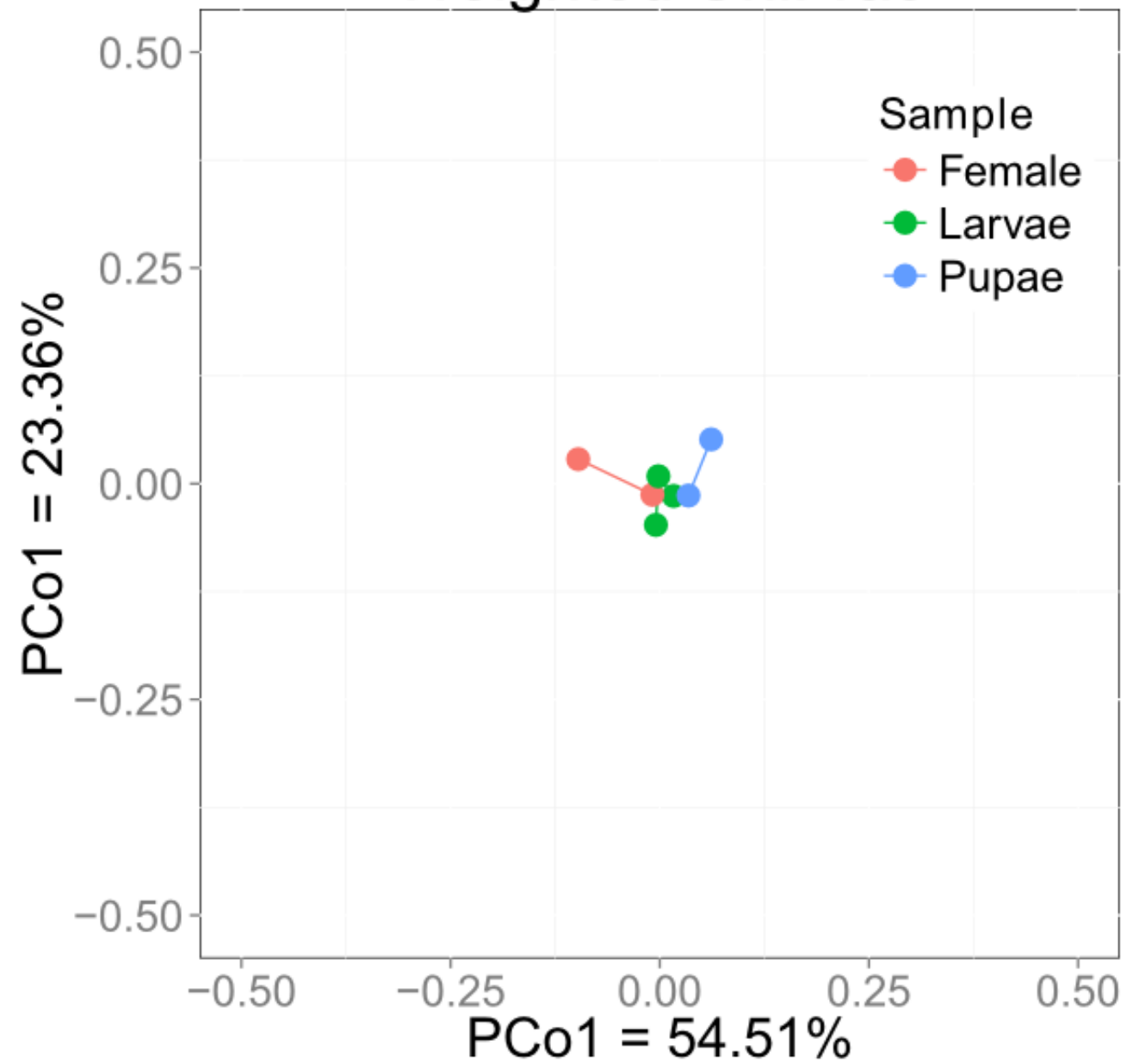
Weighted UniFrac
