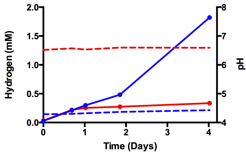
Figure S4. Abiotic controls. Hydrogen production (solid lines) in low and high pH (dashed) sterile and sealed reactors. Graphite granule cathodes were poised at -600 mV vs. SHE in phosphate-buffered medium with 50 mM sodium BES and with (blue) or without (red) 100 mM acetic acid.
