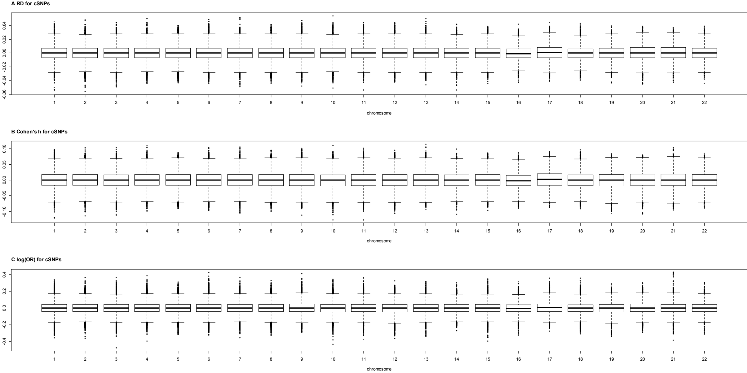
Additional file 5: Box-plot of effect sizes for common SNPs based on two shared controls in WTCCC data. Panel A: RD; Panel B: Cohen's h; Panel C: log(OR).
