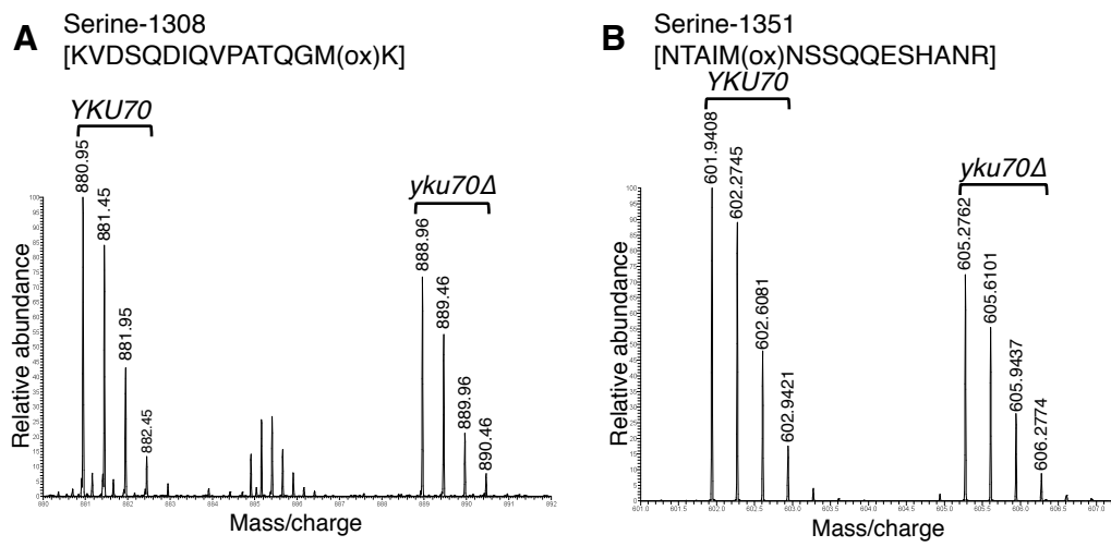
Figure S7. Abundance of non-phosphorylated Rif1 peptides is not increased in yku70Δ
