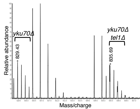
Figure S8. Abundance of a longer Rif1 peptide, phosphorylated at Serine-1308, is decreased in the absence of Tel1
