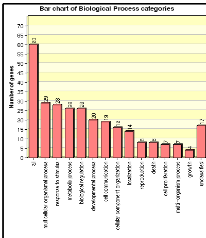
Figure S5A: GO annotation for Biological Process by WebGestalt. ( http://bioinfo.vanderbilt.edu/webgestalt/ )
