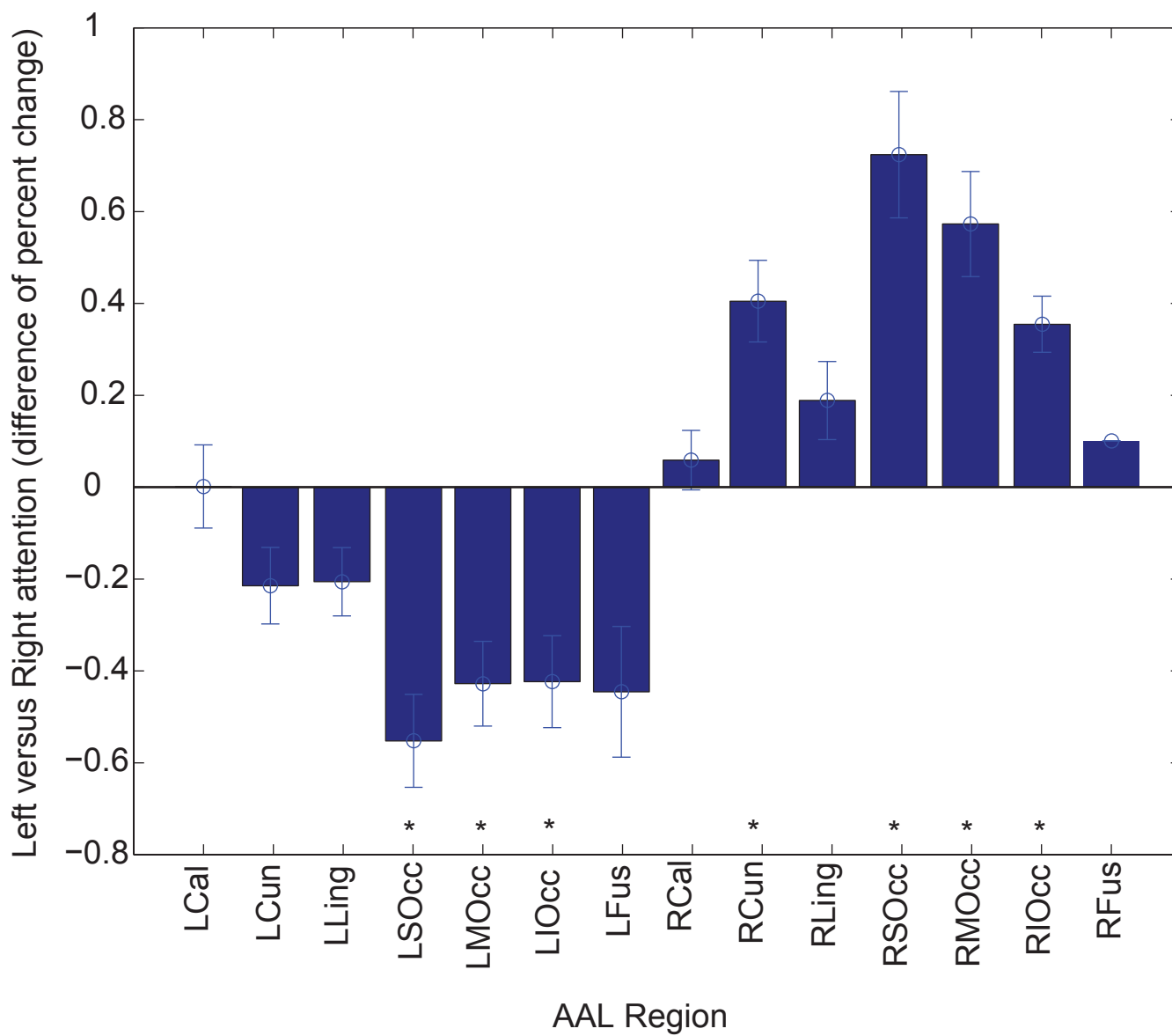
BOLD Contrast per AAL region averaged over subjects
