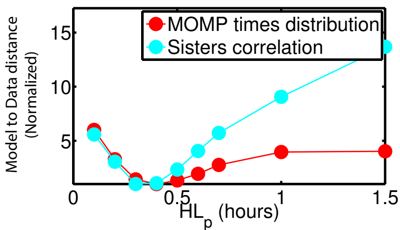
C Influence of Flip and Mcl1 protein turnover model rates on Model-Data agreement in the + CHX condition
