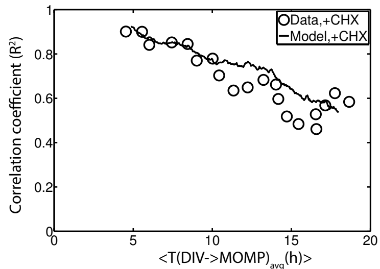
B Best Model-Data agreement for sisters MOMP time correlation in the + CHX condition
