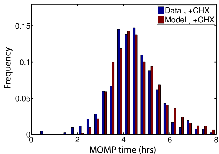
A Best Model-Data agreement for MOMP distribution in the + CHX condition
