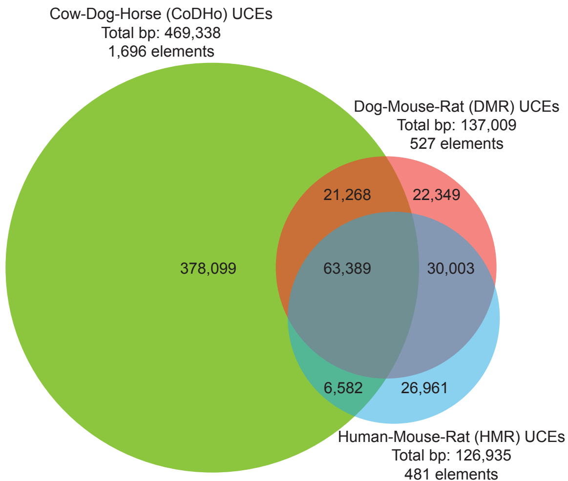
Figure S1: Intersections of the CoDHo, DMR, and HMR datasets of UCEs.
