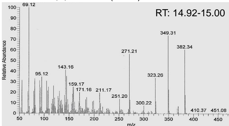
Cholesta-5,7,24-trienol (382.6)
