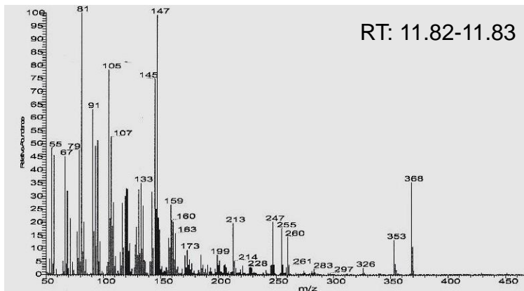
5-Dehydroepisterol (396.6)
