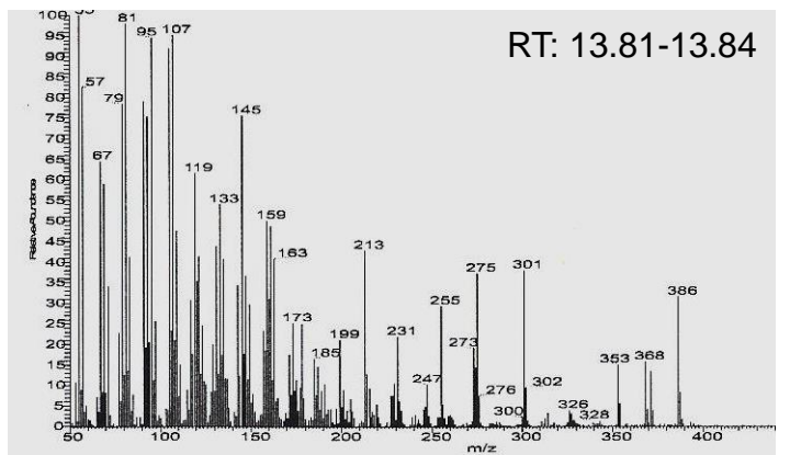
Cholesterol (386.6)
