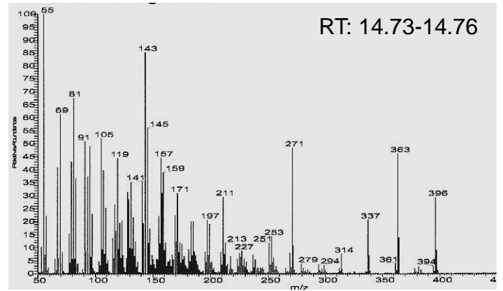
Episterol (398.6)
