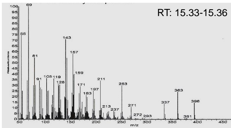
Cholesta-5,7,24-trienol (382.6)
