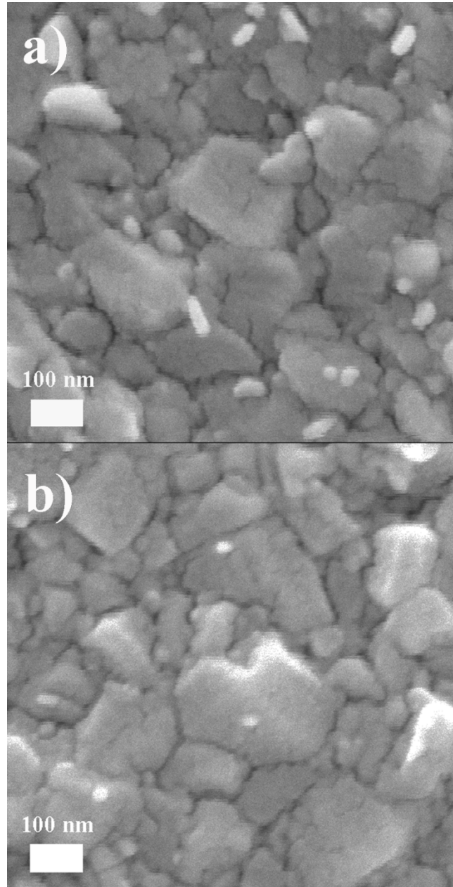
Figure S1. The SEM top-view image of the perovskite film before and after O 2 annealing process
