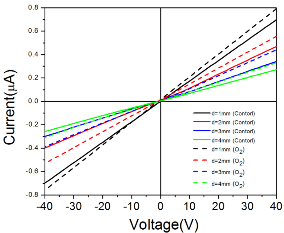
Figure S2. The I-V characteristics across the electrode with different separation on the film of spiro-MeOTAD before and after O 2 annealing
