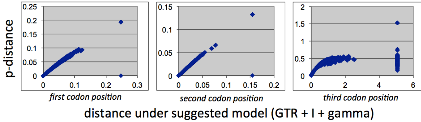
Figure S2: Distance plots showing evidence for saturation in the third position of codon in COI gene. The third position was therefore excluded from the analyses. The outlier points belong to outgroups.
