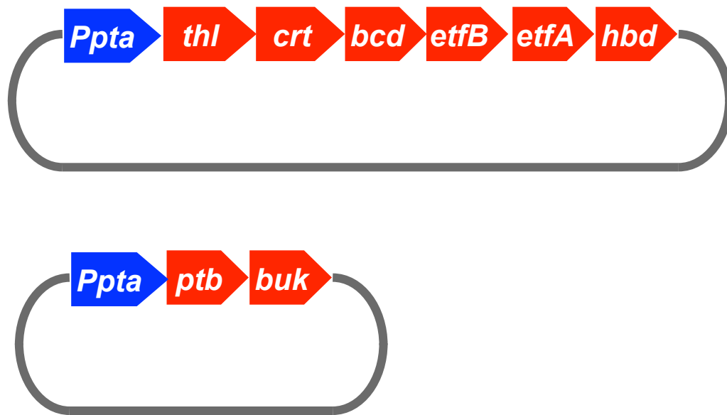
Figure S2. Plasmid vectors used for expression of the butyrate pathway genes in C. ljungdahlii to create strains B1 and B2.
